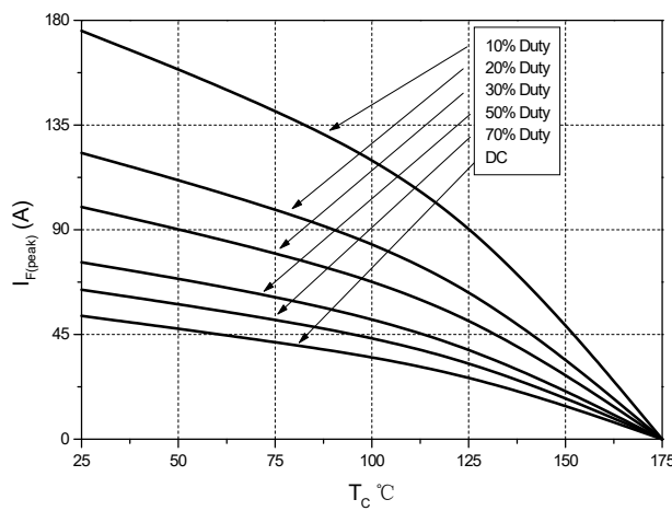
FIG.8: Current derating
