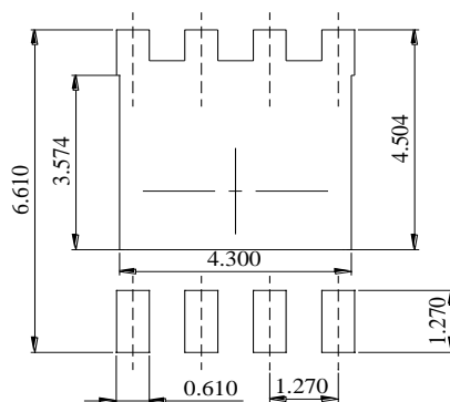
DIMENSIONS: MILLIMETERS
