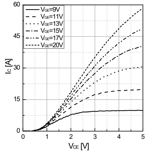
Fig 2. Typical output characteristic ( T_{vj}=150^{\circ}\text{C} )
